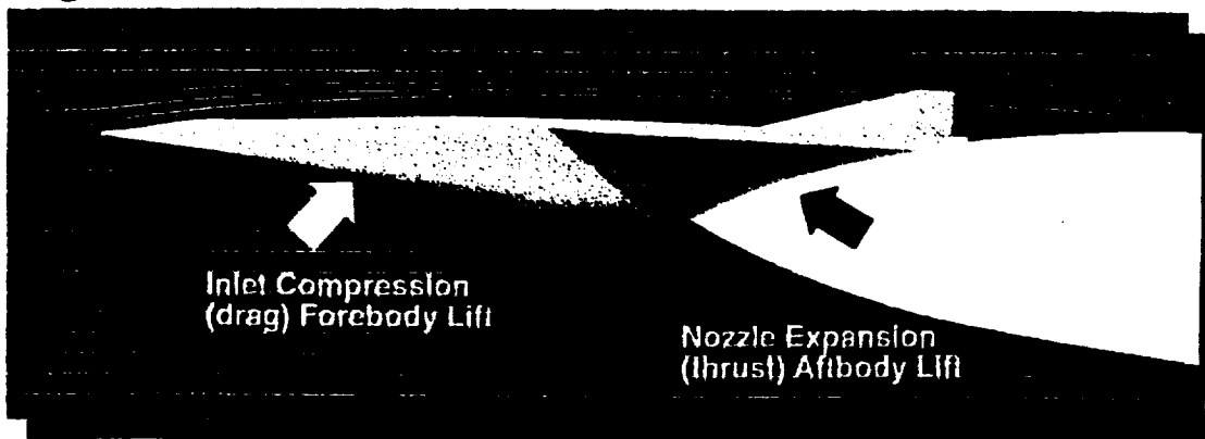
FIGURE 4. - ENGINE-VEHICLE INTERACTIONS.
