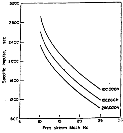
Ramjet specific impulse with supersonic burning hydrogen fuel
