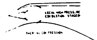
SPECTRUM OF POTENTIAL EJECTOR SCRAMJET INLET CONCEPTS
